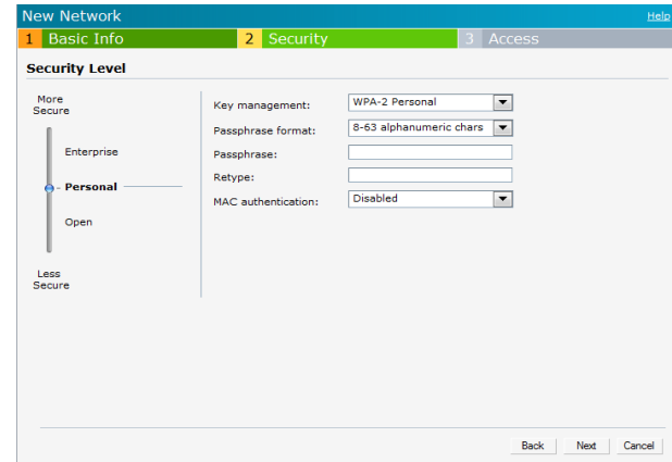
Figure 5 Security tab
